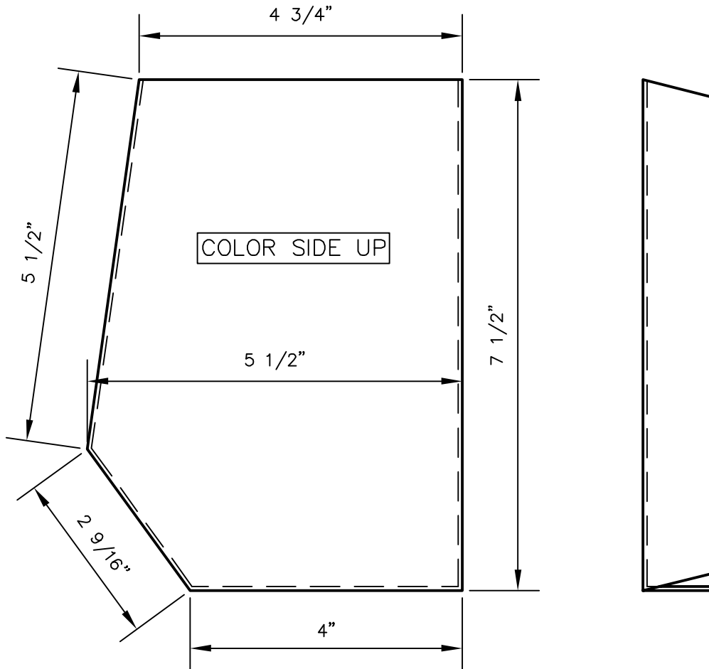
GUTTER END CAP (6:12 PITCH) - FINISHED (R.H. SHOWN - L.H. OPP.)
